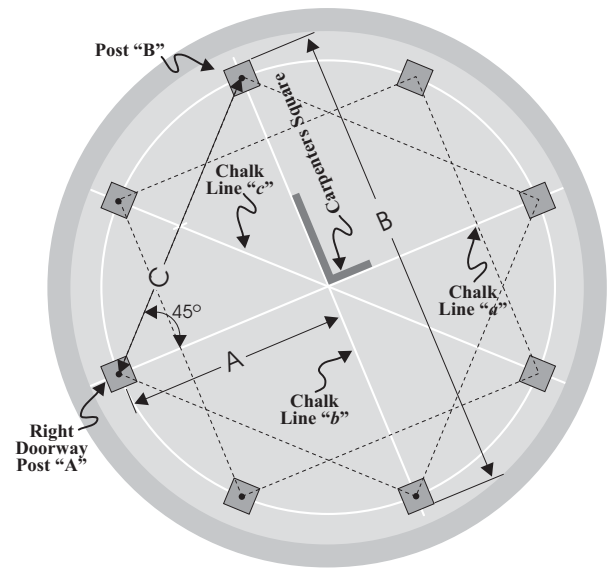
Fig. 1 Post Layout
